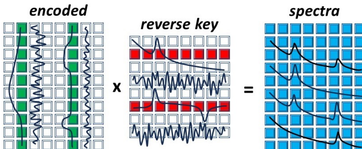
Figure 6: Inverse transformation.
