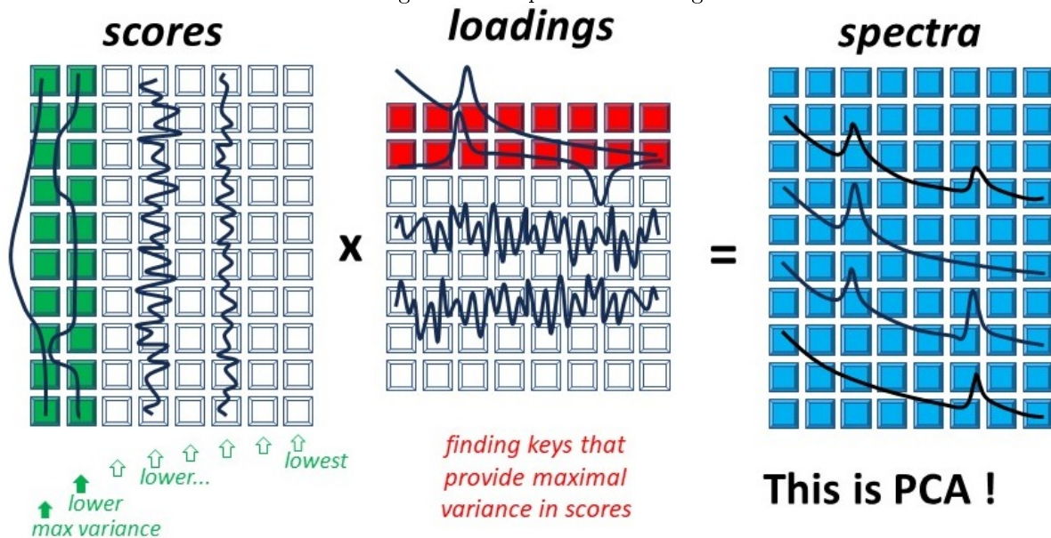
Figure 7: Compressed encoding.
